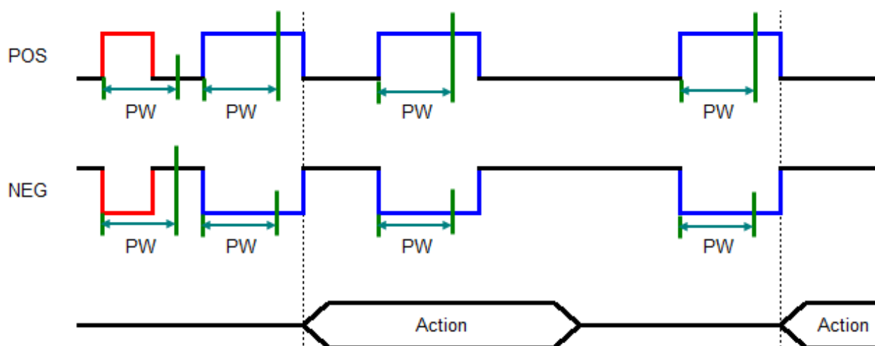
GPIO Pulse Signal : A pulse is an action. (Host to printer.)
